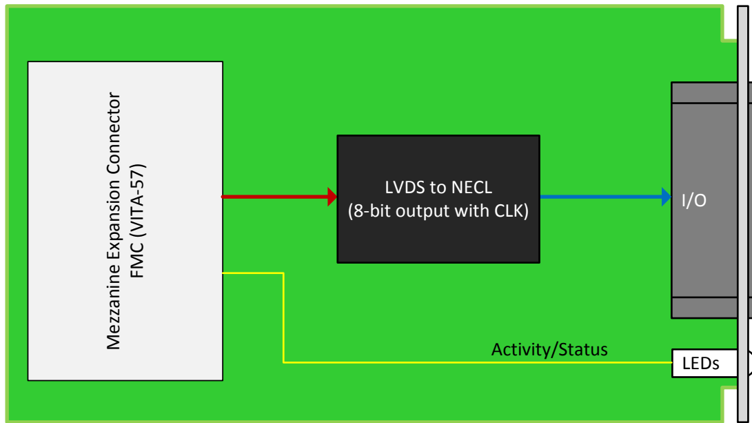
Figure 1: FMC153 Functional Block Diagram
