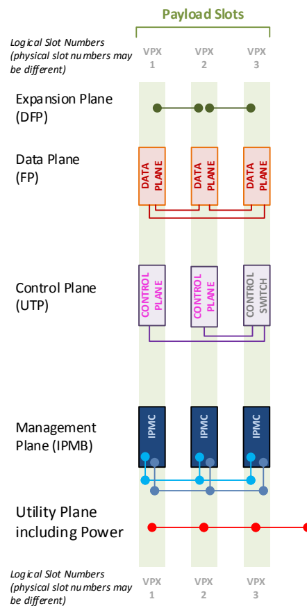
Figure 3: VTX881 Backplane Connections
