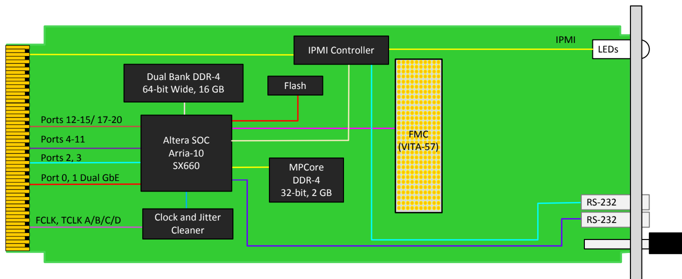
Figure 1: AMC535 Block Diagram
