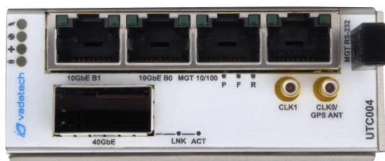
UTC004 Front panel with QSFP+ (MTCA.1)
