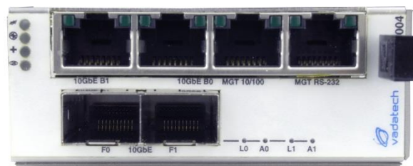
UTC004 Front panel with dual SFP+ (MTCA.1)
