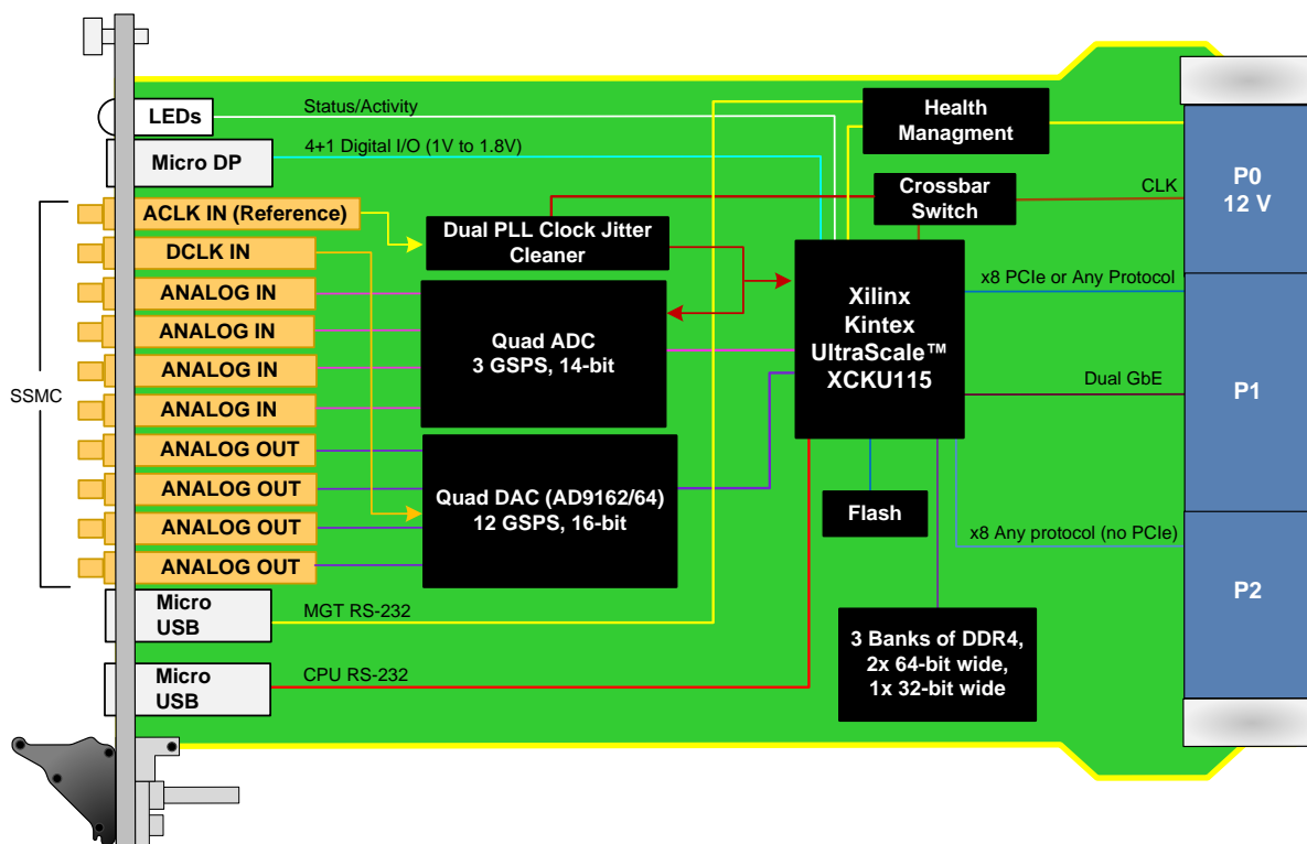
Figure 3: Functional Block Diagram for Option A=2,3
