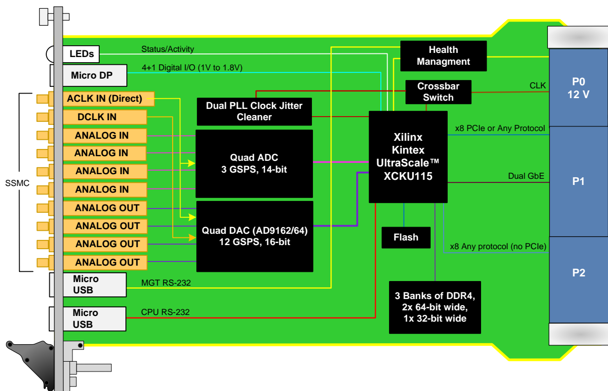
Figure 2: VPX598 Functional Block Diagram for Option A=0,1
