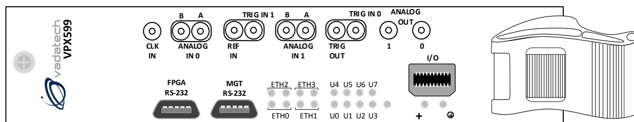
Figure 3: VPX599 Front Panel
